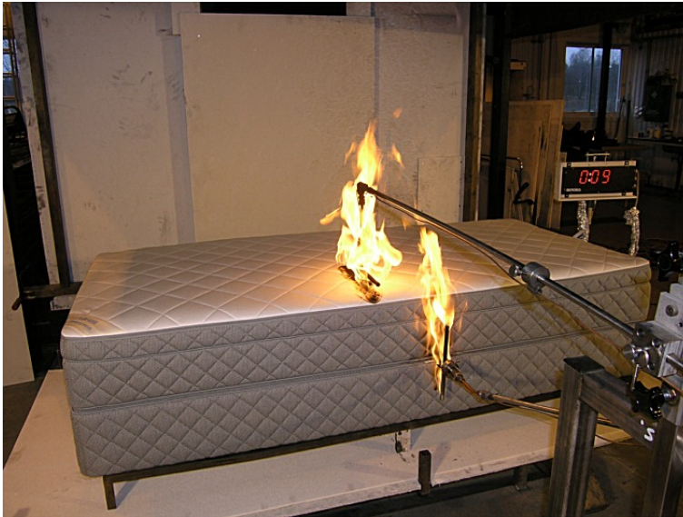
Figure I- 5 During testing according to 16 CFR Part 1633 a mattress is exposed to two T-shaped burners with a total burner heat output of 27 kW. During the test the heat release rate and the total energy developed are measured.
