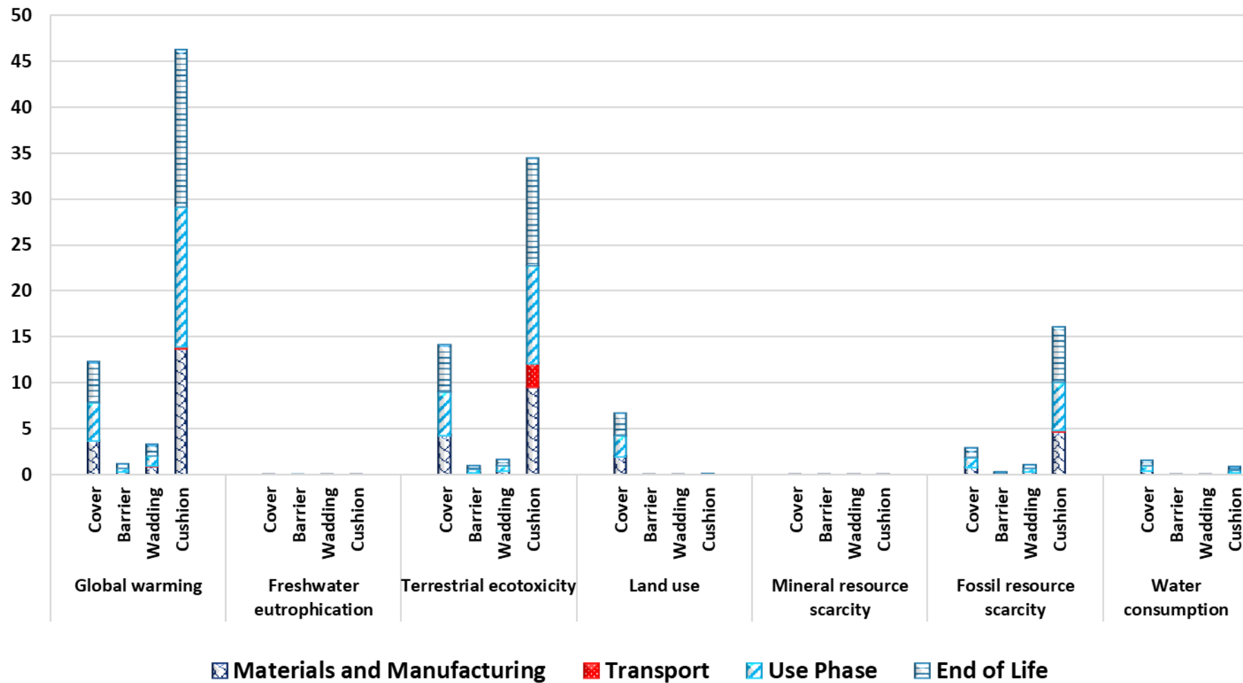
Figure G-15 Comparison of selected environmental impact categories resulted from cover, barrier, wadding and cushion parts of a loose furnishing (per 1 m² of the material ) at four stages including material and manufacturing, transport, use phase and end of life stages.
