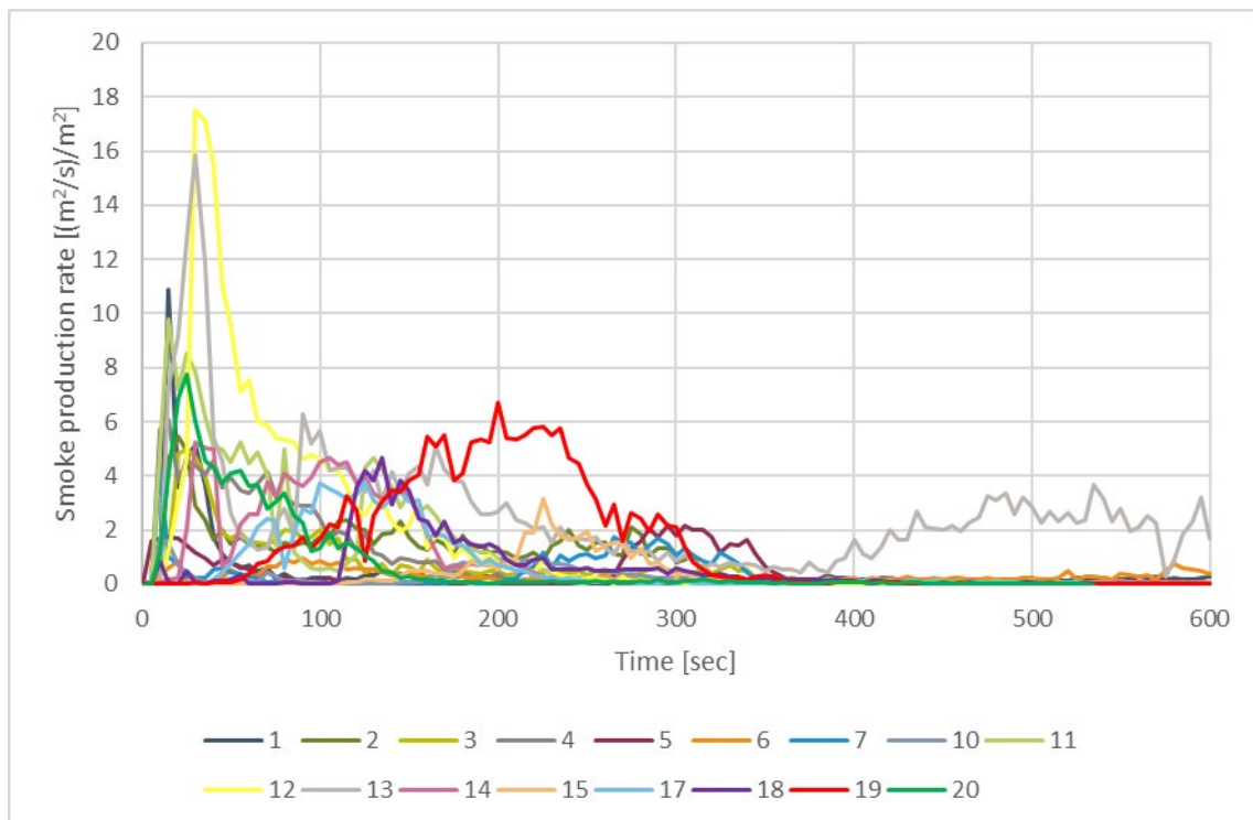
Figure 6-2 Smoke production rate, various material combinations. For specimen ID, see Table 6-1.
